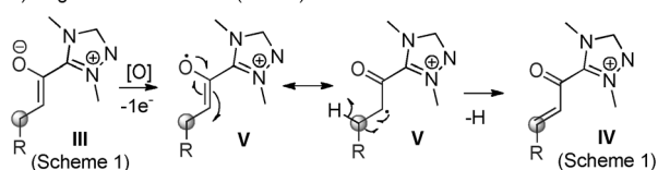
a) single-electron-transfer (radical) mechanism:
